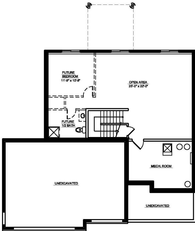
FOUNDATION PLAN
